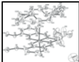
Fig. 1. A view of complex (I), showing 30% probability displacement ellipsoids and the atom numbering scheme. H atoms have been omitted for clarity.
